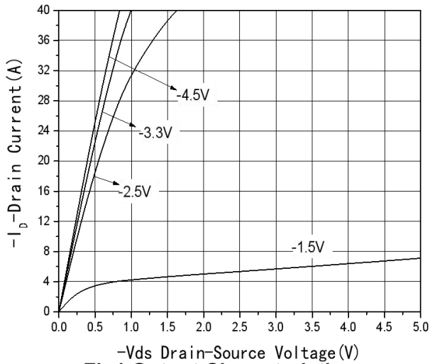
Fig1 Output Characteristics
