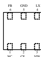
DFN2020-6L (TOP VIEW)
